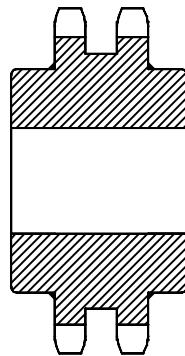
C型双排链轮 C Type double wheels
