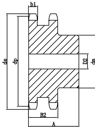
A型双排平片链轮 A type duplex plate wheels
