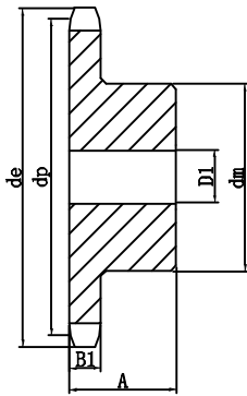
B型单排链轮 B Type single wheels
