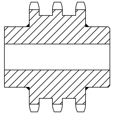
C型叁排链轮 C Type triple wheels
