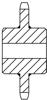
C型单排链轮 C Type single wheels
