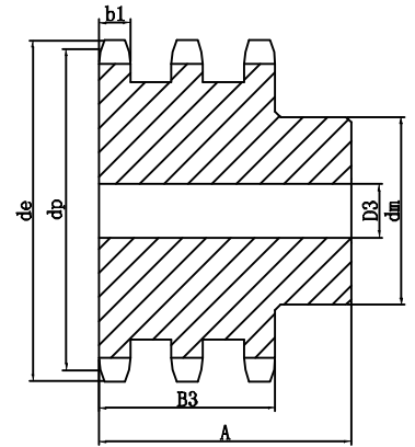
A型叁排平片链轮 A type triplex plate wheels
